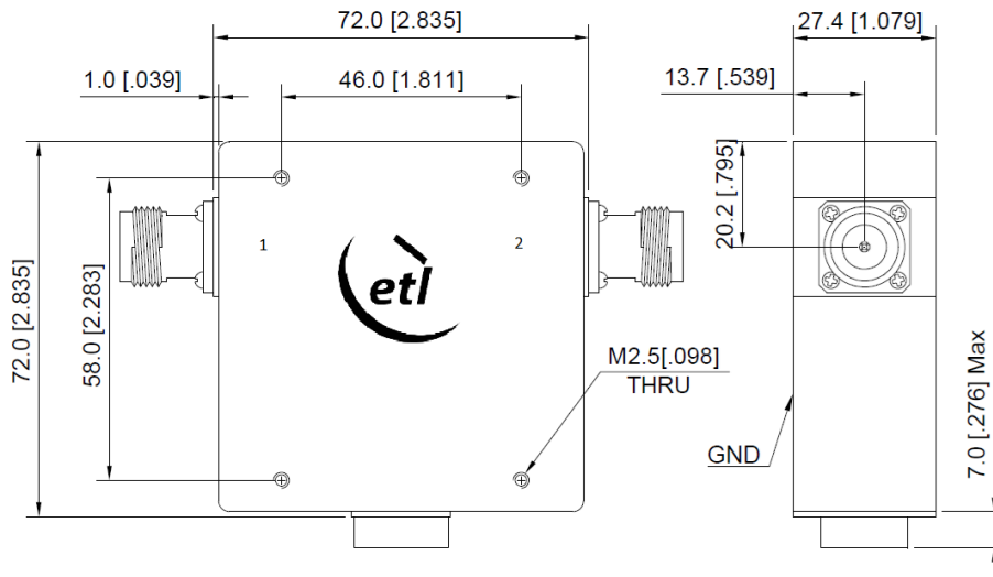
Dimensions (mm)
